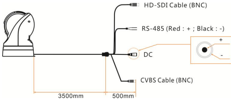
Fig. 9: Cable Package
