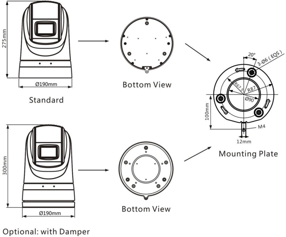
Fig. 4: Fixed Mounts (with and w/o damping system)
