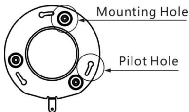
Fig. 6: Installation Plate
