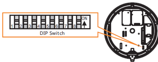
Fig. 1: DIP Switch
